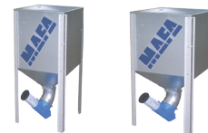
3.6 ton capacity Flexi-Bulk silo with posts and beams (not included). Specify auger or vacuum for transport from silo to boiler. Optional single fill connection at bin requires bringing fill hose to bin (as shown). Fill connection can also be made to home exterior.
